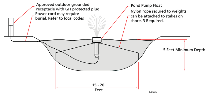
Figure 4: Typical Installation
